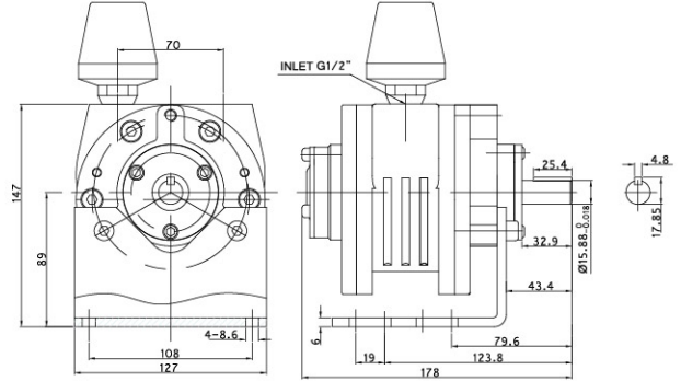
M630W Dimension Drawing
